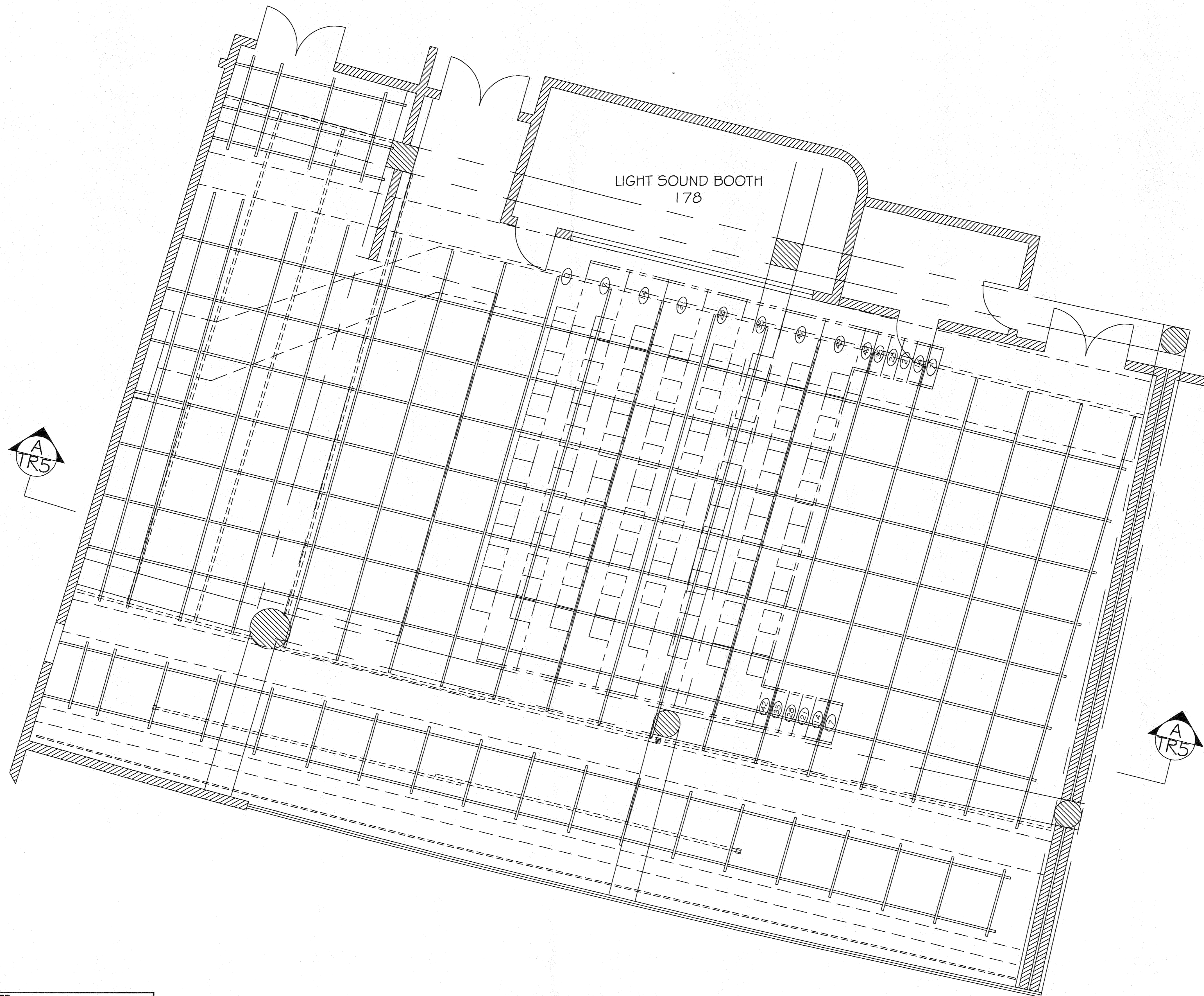
PLAN VIEW END STAGE - 112 SEATS
