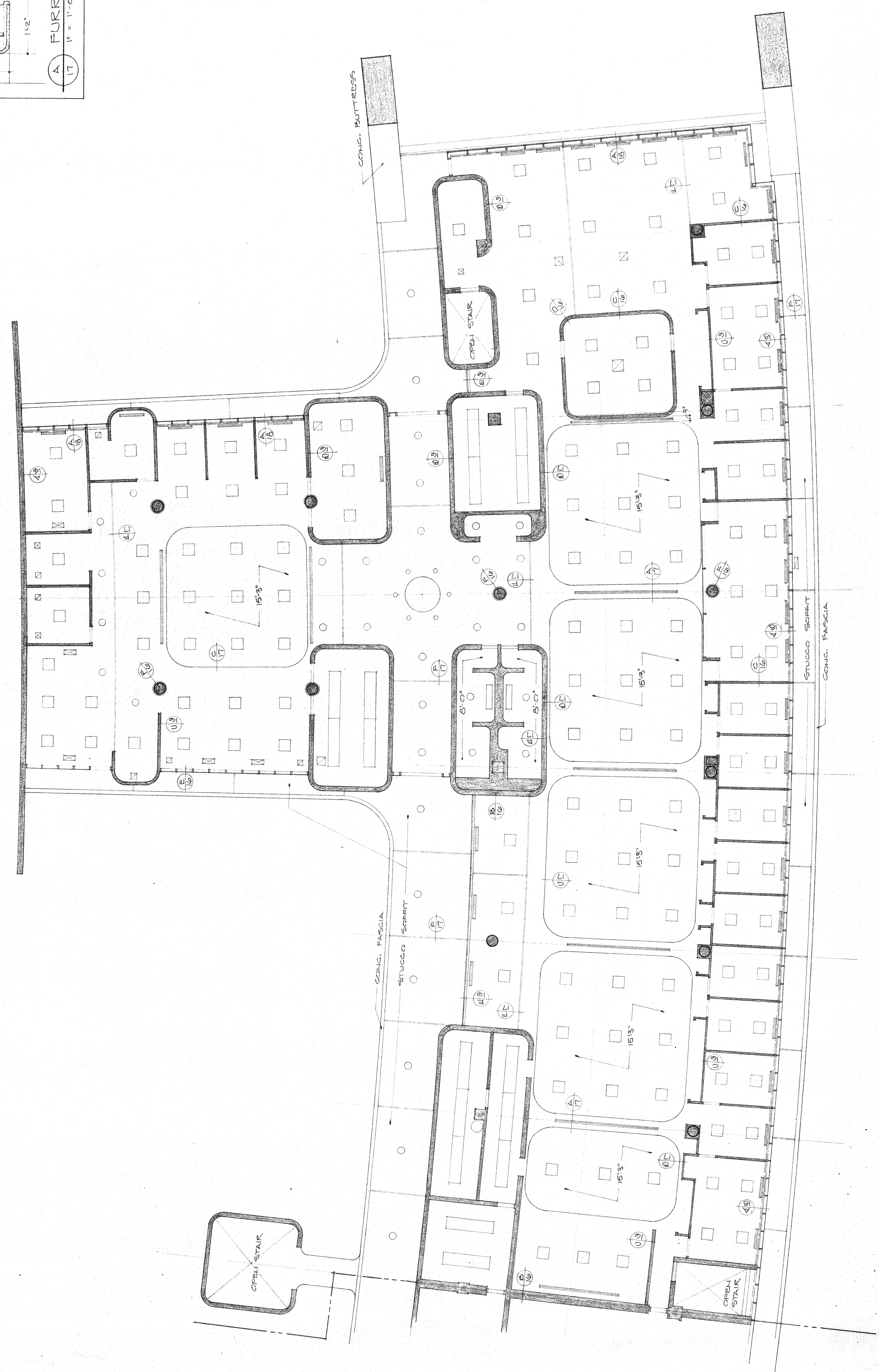
CEILING PLAN • NORTH BLDG. • SOUTH END SCALE: 1/8" = 1'-0"
